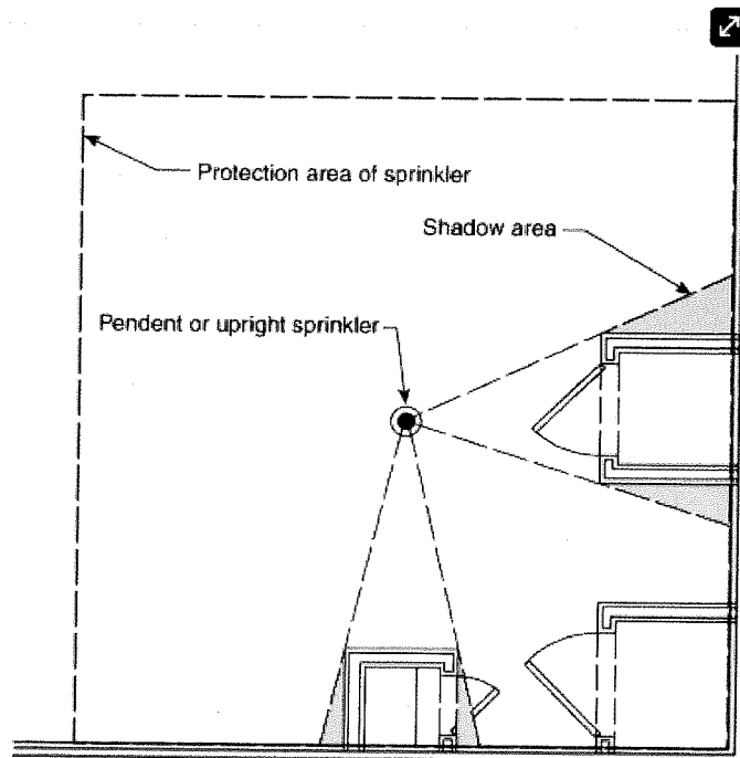
Figure A.9.1.1(3)(b) Example of Shadow Area.
